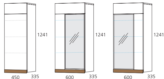
PZ-V13 L PZ-V13 D (1 VRATA / VRATA / DOOR)
